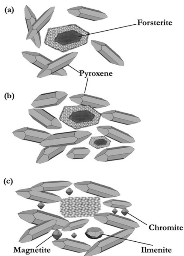
Fig. 8. Schematic illustration of the history of crystallization of minerals from forsterite to magnetite.
